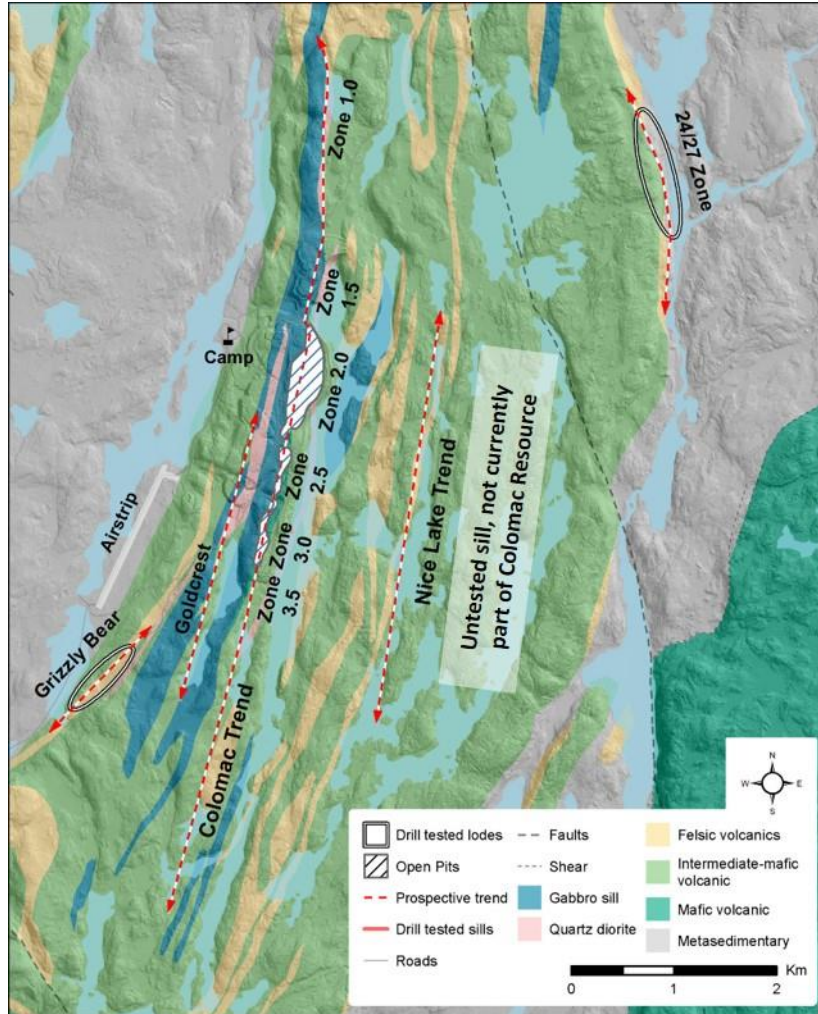
Figure 2 Deposits at Colomac Gold Project
