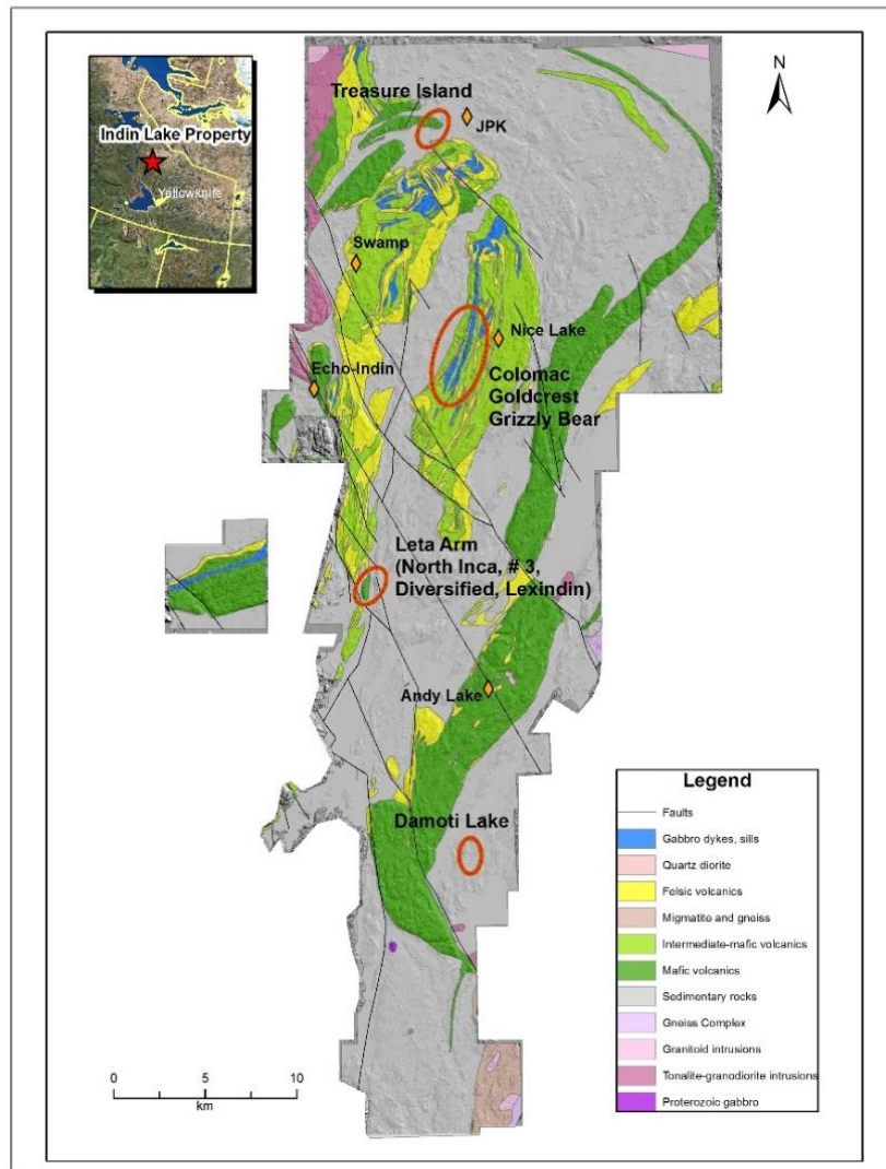
Figure 4 2018 Indin Lake Drill Targets
